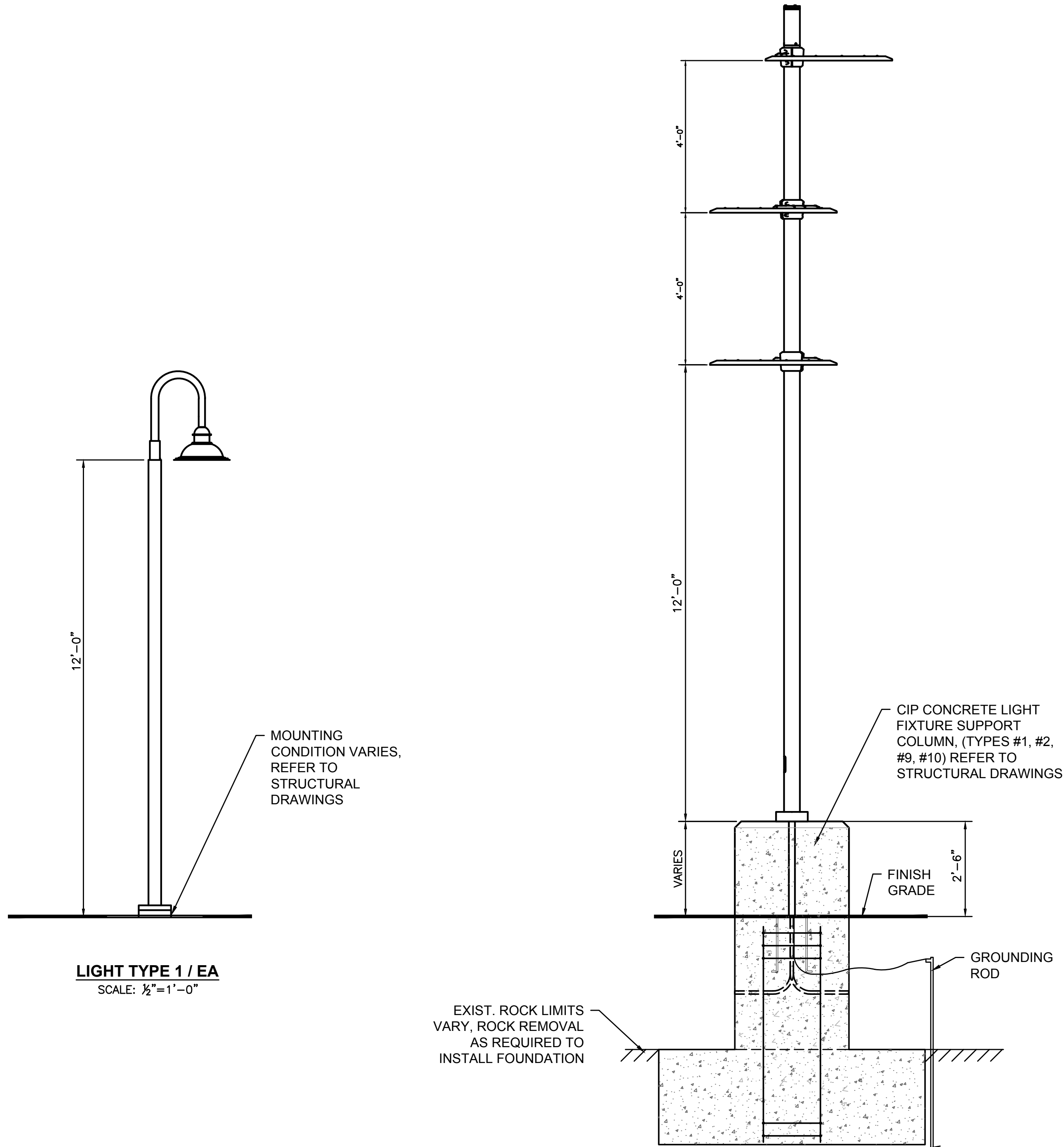
LIGHT TYPE 2 / EB SCALE: 1/2"=1'-0"
