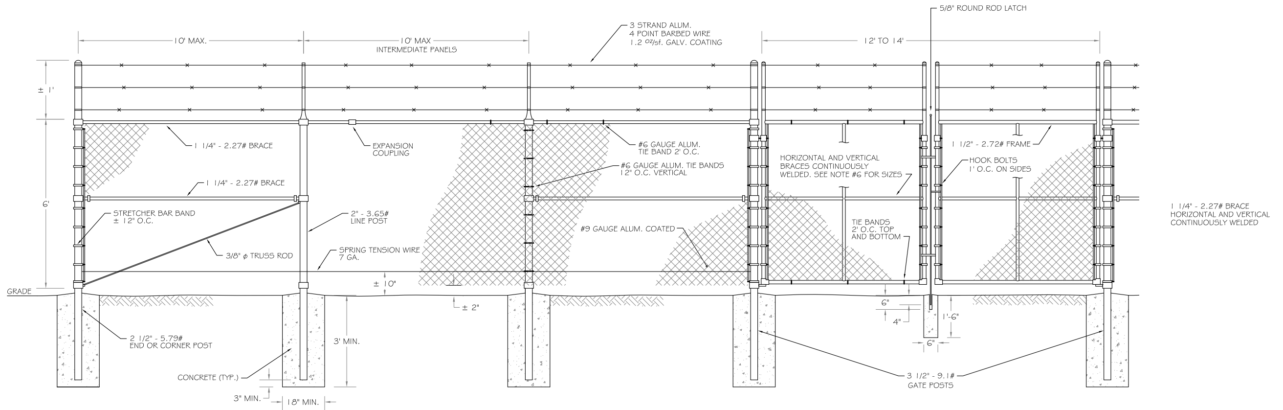
ELEVATION WITH DOUBLE GATE
