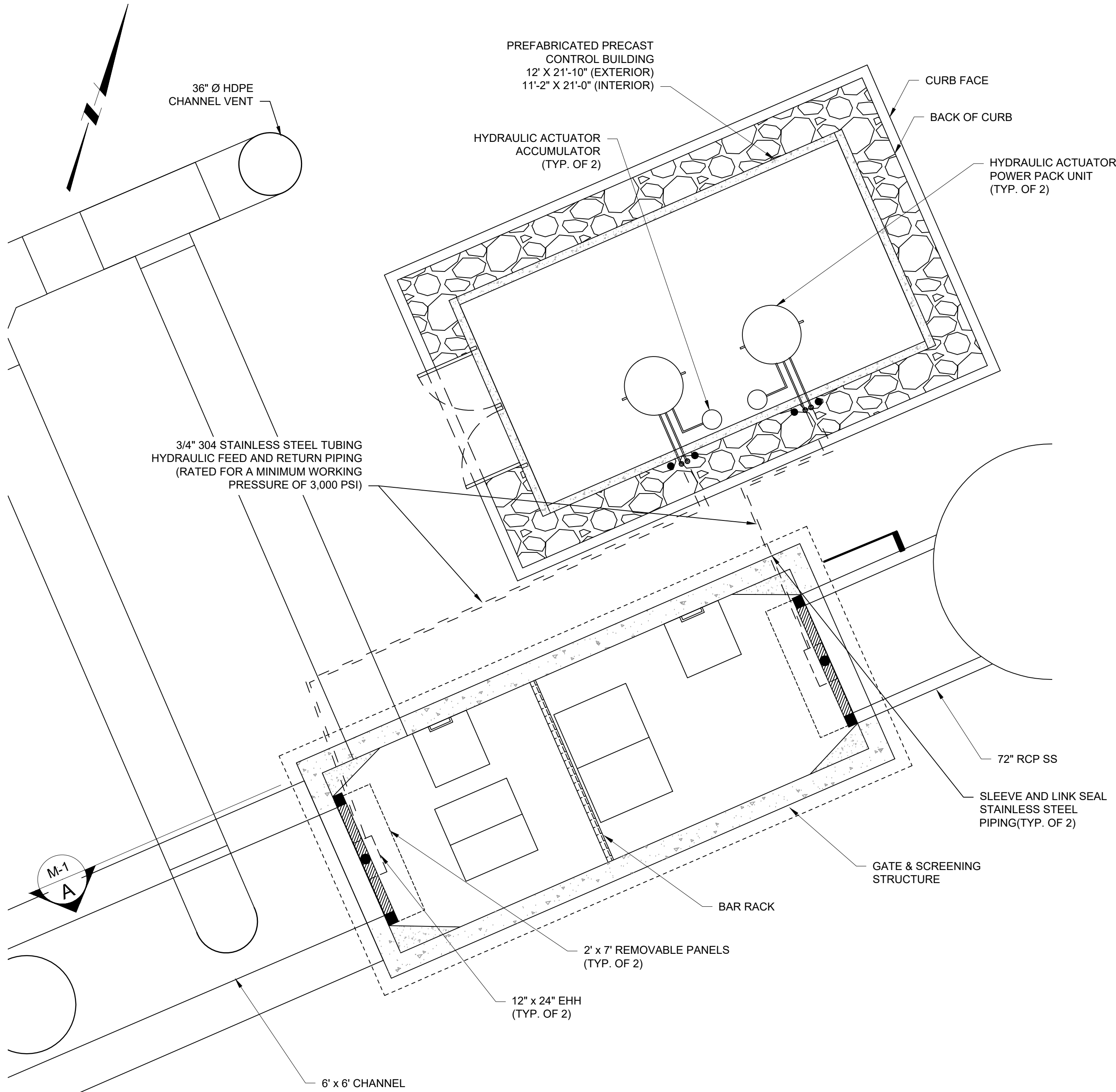
PLAN VIEW SCALE: 1/4" = 1'-0"
