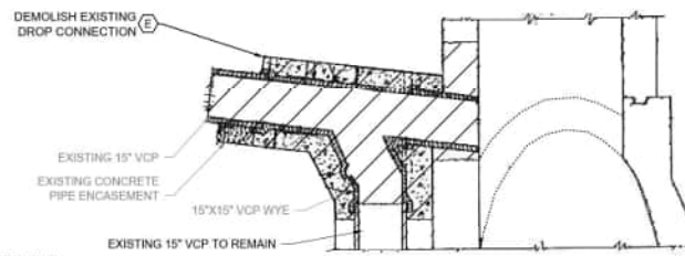
EXISTING 15" DROP CONNECTION (EX MH P210006) SCALE: NTS
