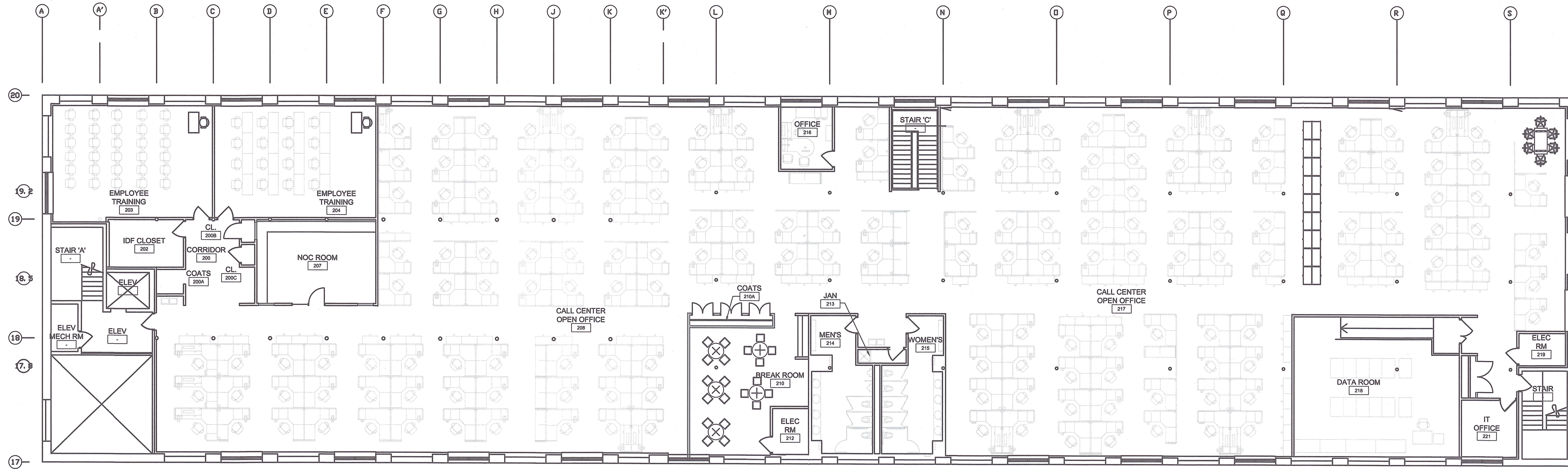
1 SECOND FLOOR PLAN
